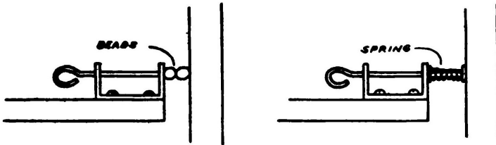
FIG. 50. Simple thrust bearing.
