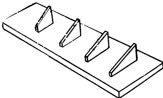
FIG. 28. Templates for testing and carving a propeller.
