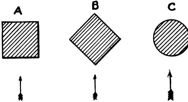
FIG. 9. Of the three shapes shown above, the round one will slip through the air with the least disturbance and resistance. A bar of wood like (A), 2 inches square, showed a "drift" of 5.16 lbs. when placed in a breeze blowing 49 miles per hour. Turning it as shown by (B) changed the "drift" to 5.47 lbs. A round bar, 2 inches in diameter, like (C) showed 2.97 lbs. "drift" under the same conditions.
