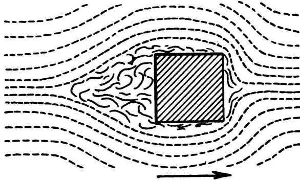
FIG. 5. The disturbance created in the air by a square object. The arrow points in the direction of motion. The space in the rear of the object is the scene of violent eddy.
