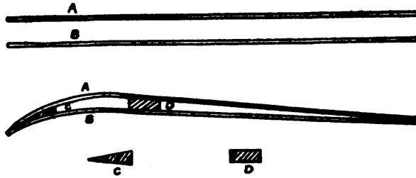
FIG. 13. Section of a built-up plane showing how a rib is made. When made small, they offer greater "drift" or head resistance than a single curved surface plane and cannot because of the delicate structure necessary to make them light, withstand hard knocks. They have the further disadvantage of being from a constructional standpoint very hard to make smooth and rigid.
