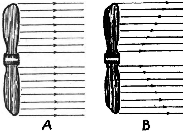
FIG. 27. A propeller of the truly helical type delivers a cylinder of air in which all parts move at the same speed as at A. A propeller having blades of the same angle throughout their length throws the air as in B in which the centre of the cylinder moves more slowly than the outside.
