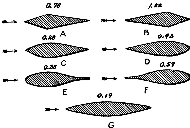
FIG. 10. The figures given above each shape show the "drift" in lbs. of wooden bars of those shapes when placed in a wind blowing 40 miles an hour. The bars experimented with had a depth of 9 inches in the direction of the arrows and were 2 inches wide.
