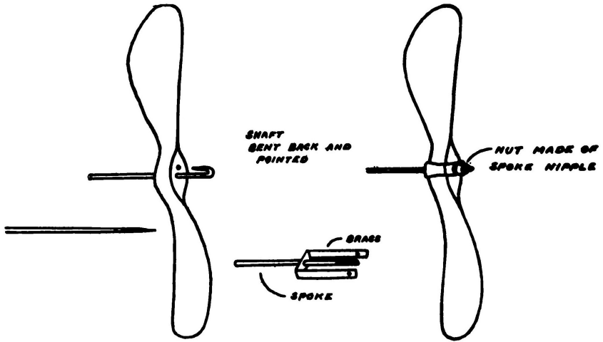
FIG. 33. Methods of fastening propellers to shaft.
