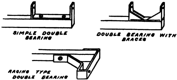
FIG. 49. Double bearings.
