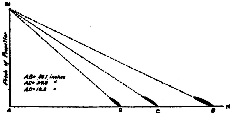
FIG. 26. Method of laying out a screw propeller, that is, determining the angle of the blades at different points.
