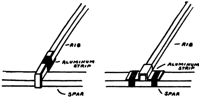
FIG. 14. How ribs may be joined to the long members.
