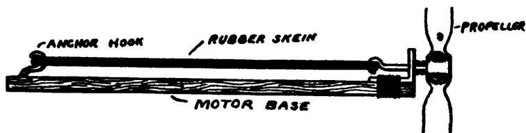
FIG. 21. A simple "motor base" or fuselage.
