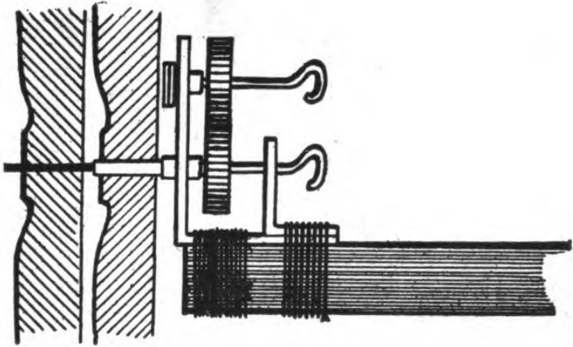
FIG. 47. A method of arranging two propellers on the same axis.
