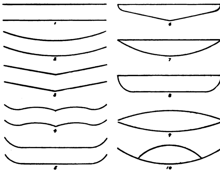
FIG. 19. The various ways two planes may be combined to secure stability or form a biplane.
