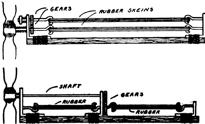
FIG. 23. Two methods of gearing a propeller.
