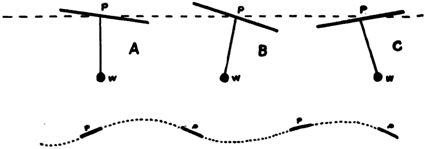
FIG. 45. Accentricity. The effect of placing the center of gravity too low.
