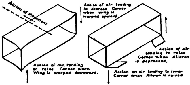
FIG. 4. Two methods of controlling the lateral stability of an aeroplane.
