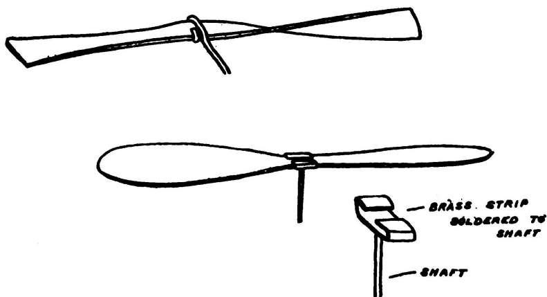
FIG. 35. Bent wood propellers and the methods of fastening them to the shaft.
