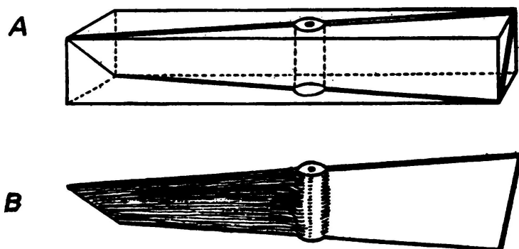
FIG. 32. Method of carving a propeller of the truly helical type.
