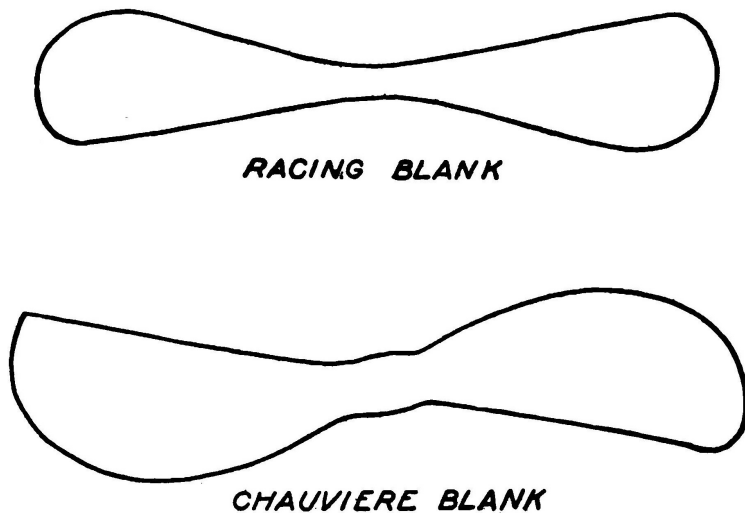
FIG. 39. Blanks for racing (top) and chauviere (bottom) propellers.
