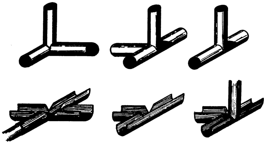
FIG. 34. Method of forming sockets for joining struts, etc., by cutting from sheet metal.
