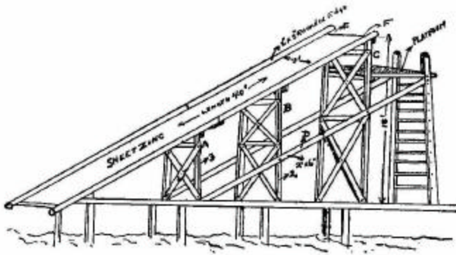
DIAGRAM FOR "CHUTE" Diagram For "Chute"
