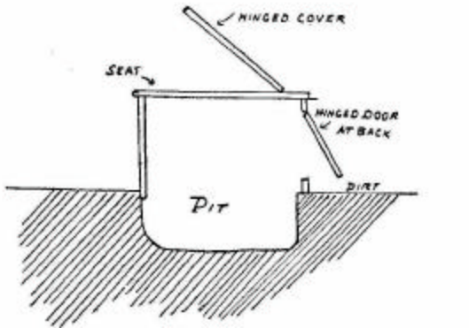
Pit Toilet; seat, hinged cover, hinged door at back.
