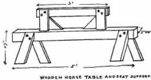
Wooden Horse Table and Seat Support
