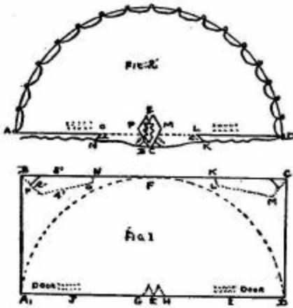
THE TEN FOOT TEEPEE
