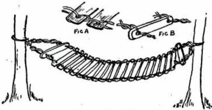
ROUGH AND READY HAMMOCK
