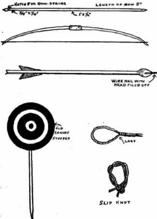
Notch for Bowstrings; Length of Bow 5 feet. Wire nail with head cut off (arrow head) Old Canvas Stuffed (target); Loop (in bowstring); slip knot.
