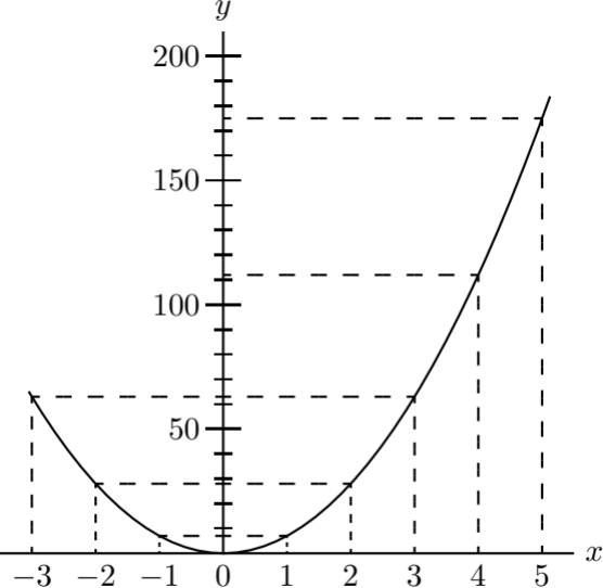
FIG. 6.—Graph of y = 7x^2 .
