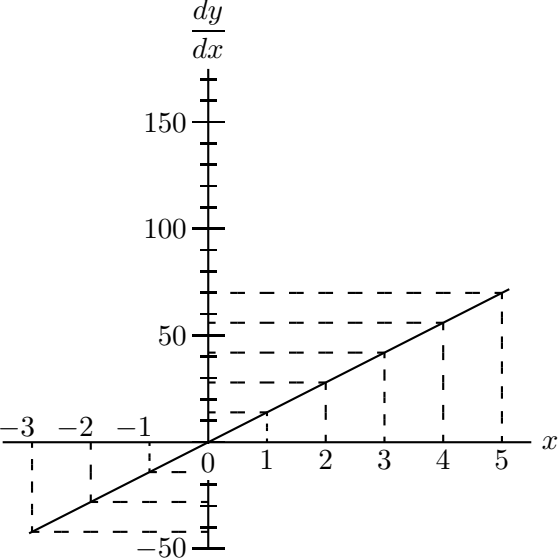
FIG. 6a.—Graph of \frac{dy}{dx} = 14x .
